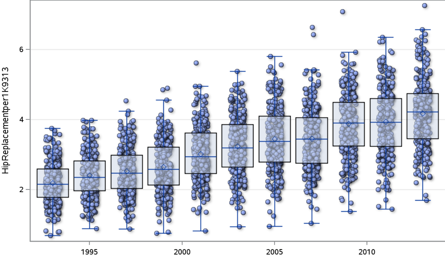
This graphs uses jitter on discrete X axis
