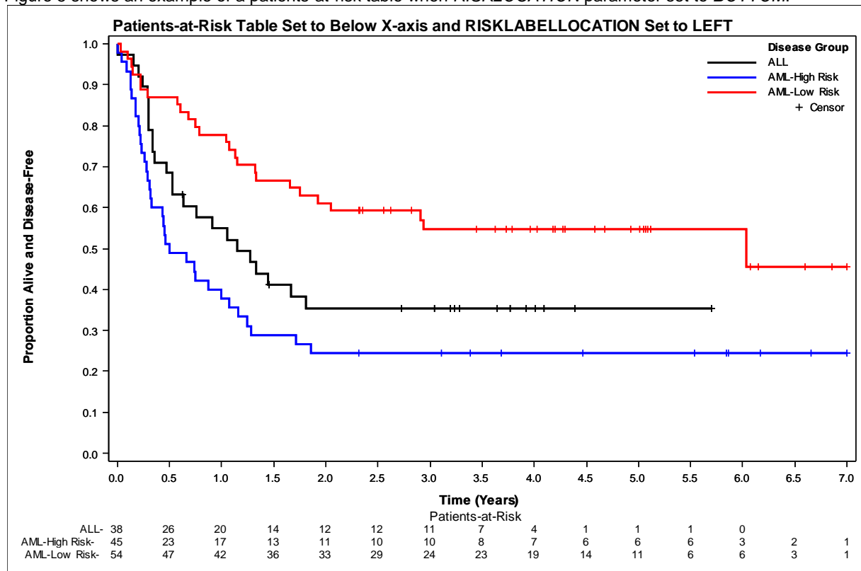
Figure 5. Patients-at-risk table displays one row per CLASS variable level in the same order as the in plot summary table.
